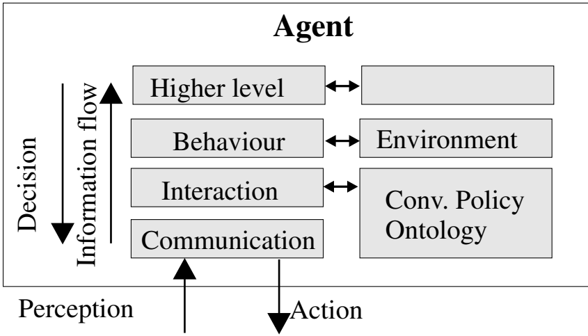
Fig. 2. General agent architecture
