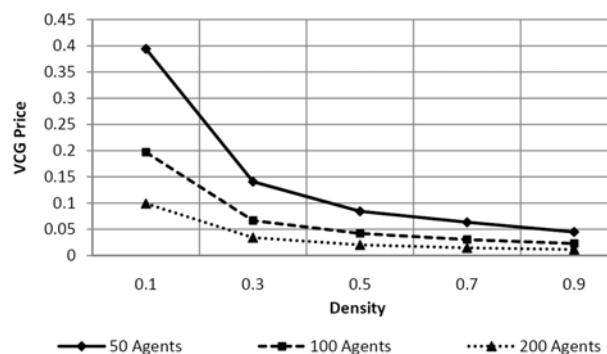
Figure 9: Mean path prices in VCG
