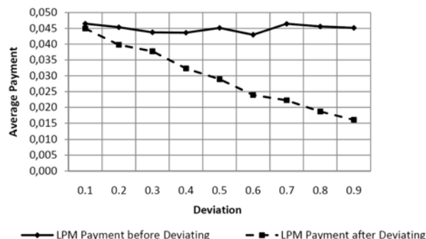
Figure 11: Mean Payment to Agents in an LPM
